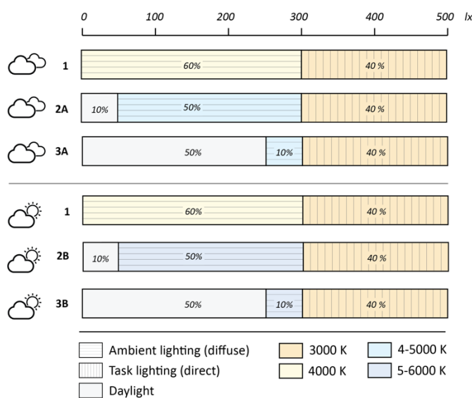
Fig. 4: The illustration is representing the standard light settings for the DDL concept. The light setting 1 is designed for the dark and transition hours, when the daylight inflow is >50 lx. This value is dependent of the architecture of the space and where the daylight measurements are made. The settings 2a and 3a are designed for overcast sky condition with different light levels and 2b and 3b accordingly for clear sky condition. See Research Paper 4 for prior field study and lighting settings.
